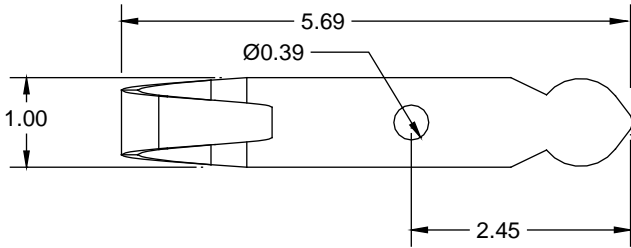
RAT TAIL HOLDBACK
