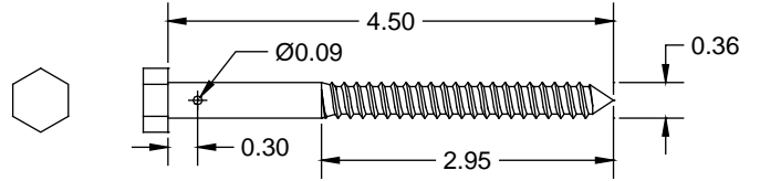
SHUTTER HOLDBACK BOLT
