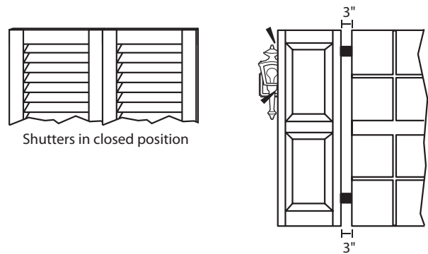
Ensure proper clearance of shutters.
