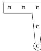
6" L-Hinge Back Plate
